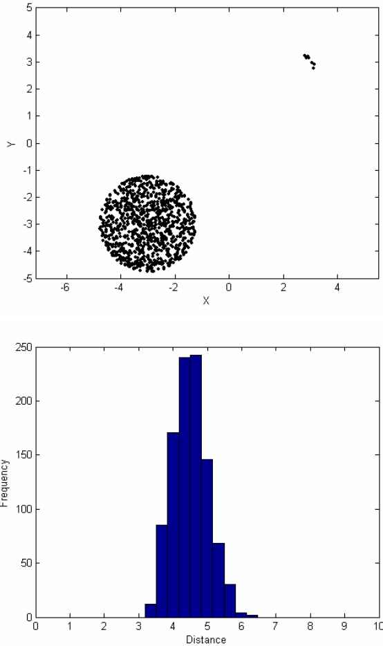
Figure 3. Sampling on the 2D (top) and 10 D (bottom) f_{Sumcan2} .
